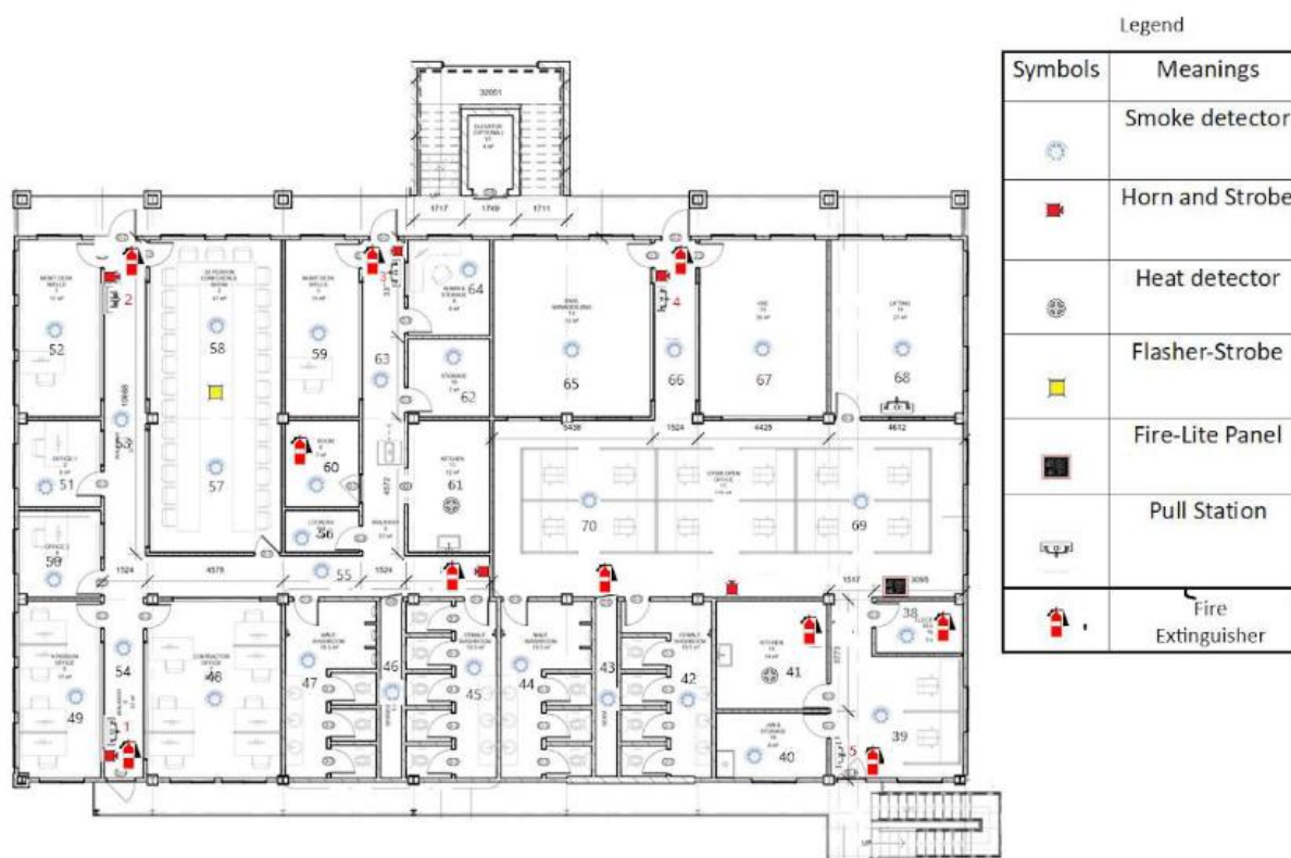
Figure 1. First Floor Fire Alarm Layout
